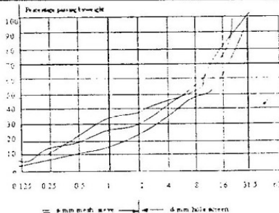
Figure 2: Aggregate grading curve
