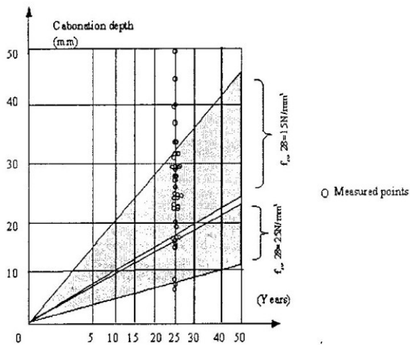
Fig. 1 Depth of carbonation according to the resistance of 28 days old concrete.
