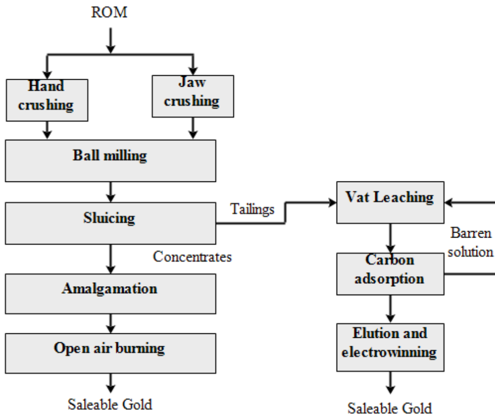
Figure 6: Current practices of gold processing at ASGM in Tanzania.
